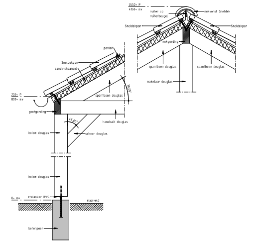
DETAILS 1: 20
